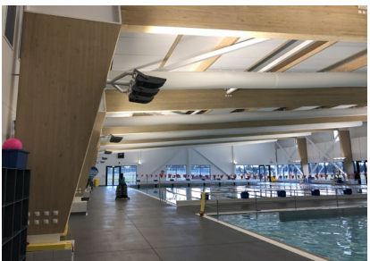
30m Span Glulam Portals
