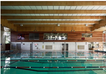
26m Span LVL Box Beams
